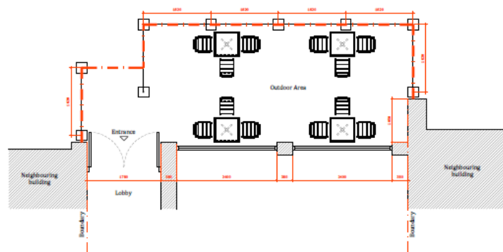
Proposed Outdoor Area 1:50 @ A3
