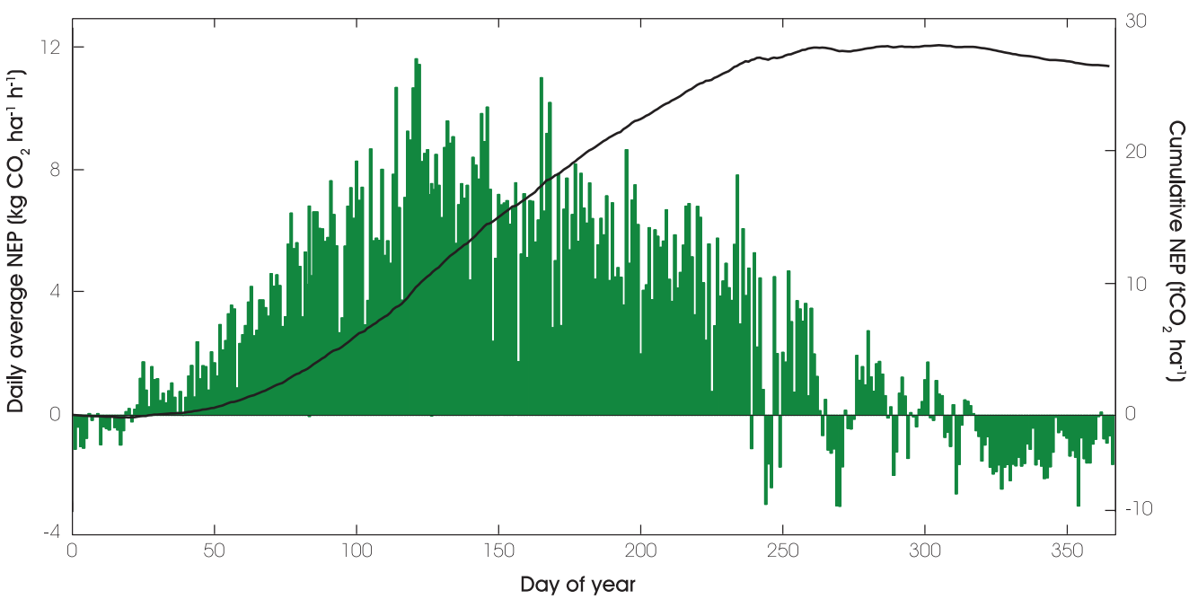
Figure 2a The daily average (over 5 years) net removal (positive) or release (negative) of CO 2 from (to) the atmosphere by a 17 to 21 year-old stand of Sitka spruce at Griffin Forest, Scotland between 1997 and 2001. Values are expressed as kg CO 2 per hectare per hour, i.e. Net Ecosystem Productivity (NEP). The vertical columns show the daily (24 hour) net CO 2 fluxes for every day of the year. The columns above the zero line show the net 24h removals from the atmosphere and gains by the forest, while those below the line indicate the net daily emissions from the forest to the atmosphere. The solid line shows the five-year-average of accumulated removals from the atmosphere.
