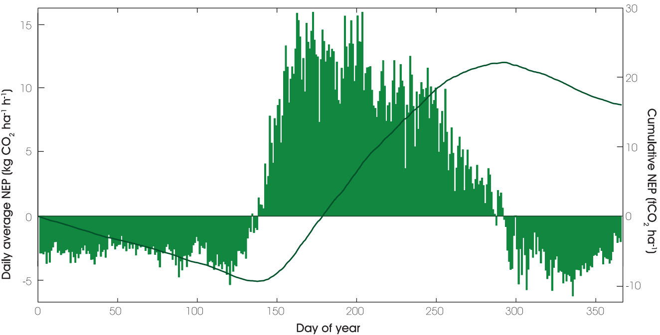
Figure 2b The daily average (over 8 years) net removal (or release) of CO 2 from the atmosphere by a 72 to 80 year old mixed oak–deciduous woodland at the Straits Enclosure, Alice Holt, England between 1999 and 2006. Other details as in (a) above.
