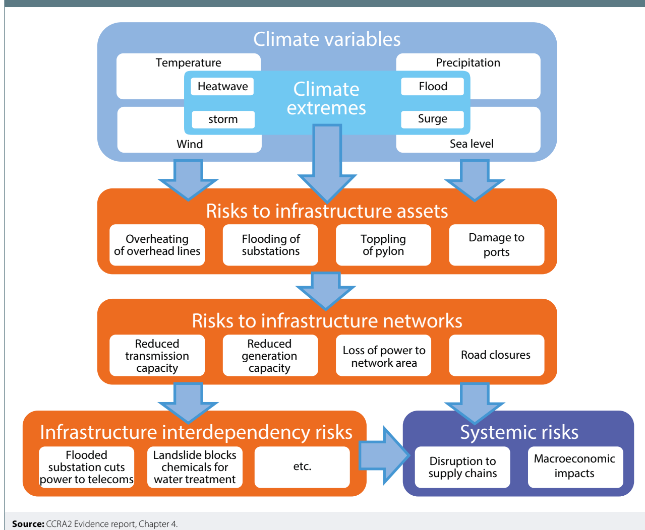
Figure SR.A2: Example relationships between climate variables and infrastructure impacts
