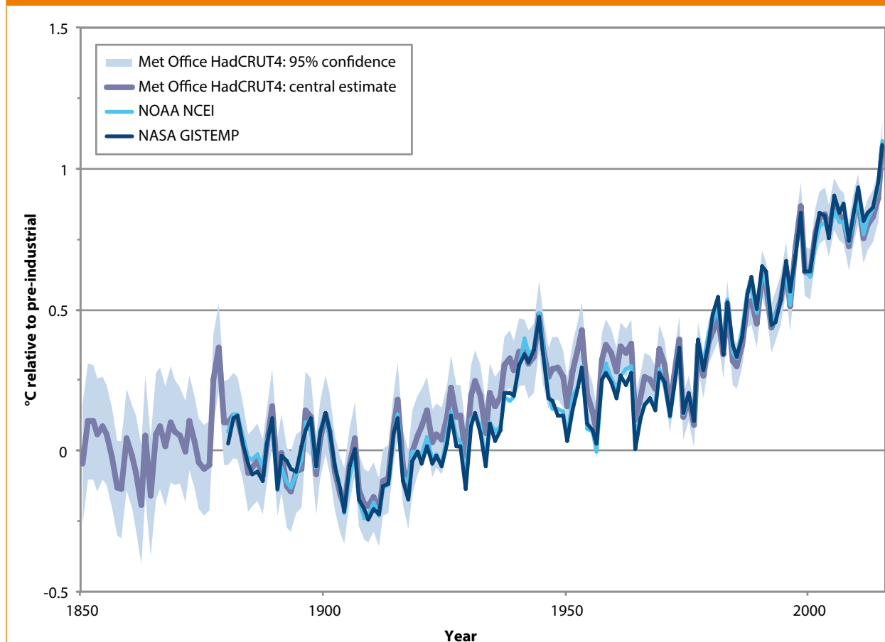
Figure SR.3: Global average surface temperature since the mid 19th century
