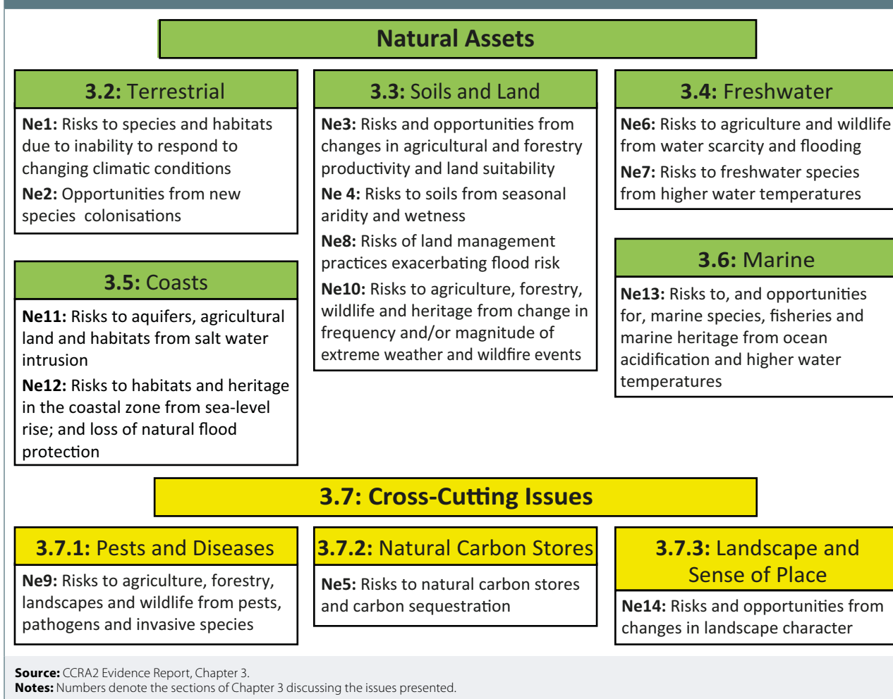
Figure SR.A1: Climate change risks and opportunities for the natural environment
