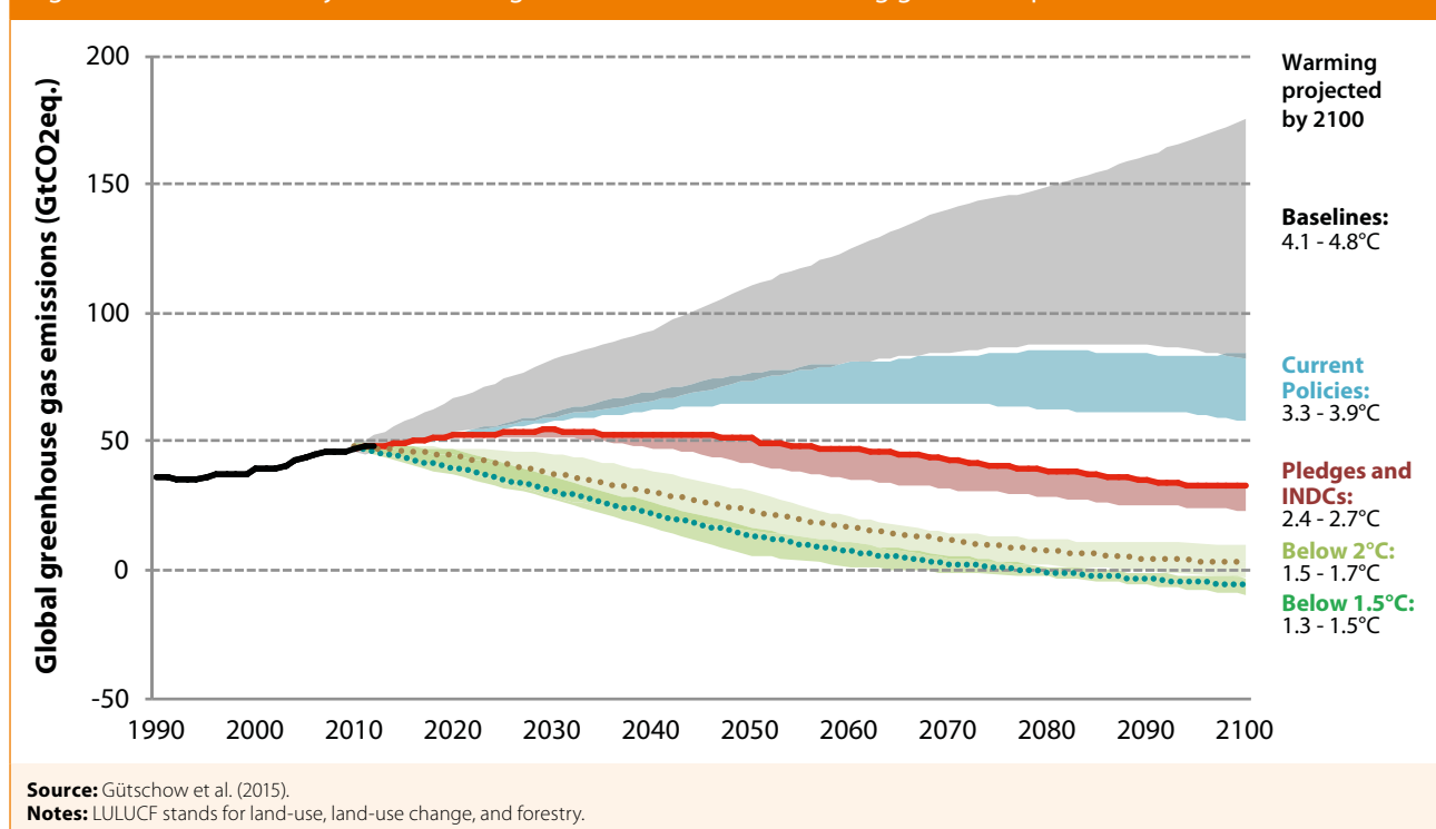
Figure SR.4: Potential trajectories of long-term emissions and resulting global temperatures
