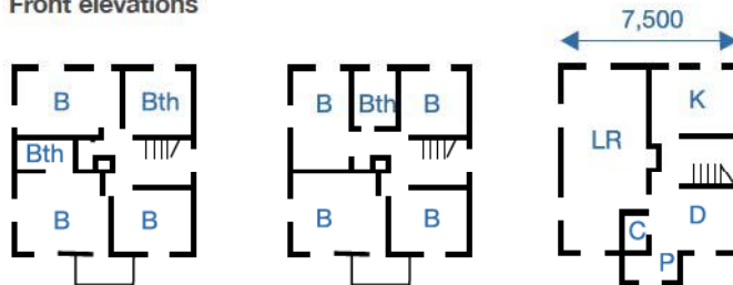
Alternative first floor
