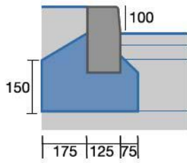
Upstand Kerb to road Types 1, 2 and 3
