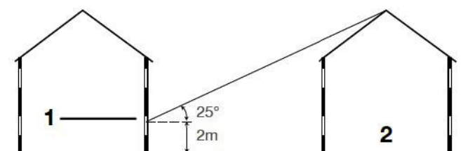
1. Reference line for daylight calculation 2. Obstructing building
