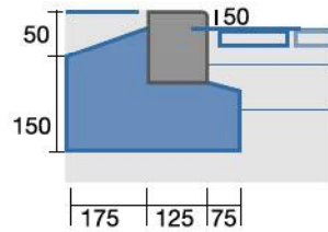
Edge detail with paviors
