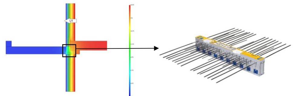
Energy flow diagram produced for a balcony to internal floor/external wall junction, produced from a Psi-value calculation. Example Schock Isokorb thermal break was tested to mitigate this thermal bridge.
