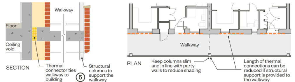
Diagram illustrating how to design out thermal bridges on access walkways. Source: Passivhaus easi-guide
