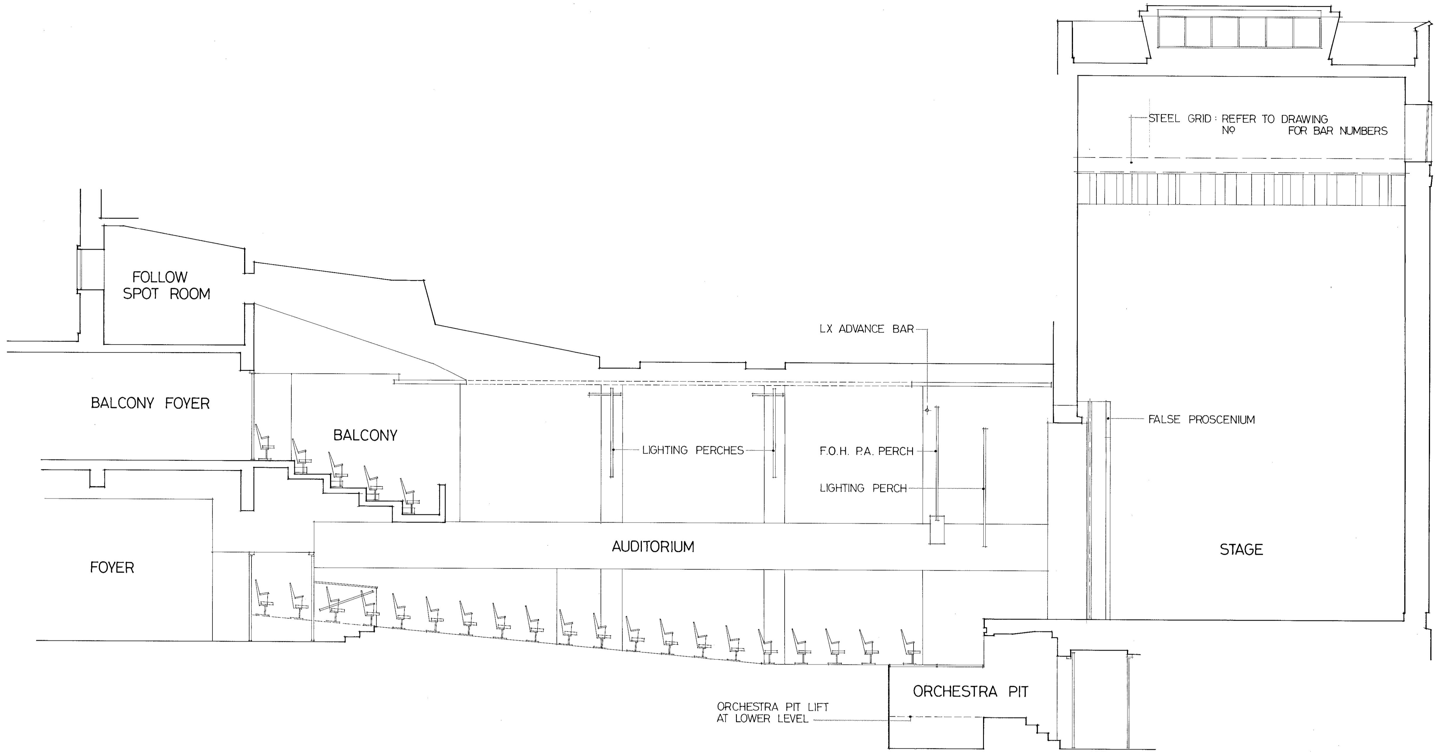
CROSS-SECTION THROUGH AUDITORIUM / STAGE
